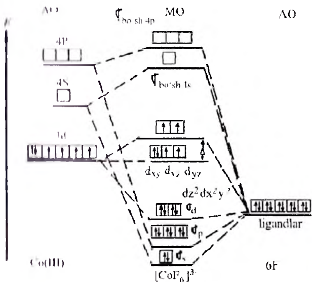
27 rasm. Molekular orbitalar usulida past spinli [\text{Co}(\text{NH}_3)_6]^{3+} va yuqori spinli [\text{CoF}_6]^{3-} komplekslarining energetik diagramlari tuzilishi.
