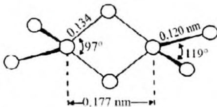
39-rasm. Boretan molekulasi tuzilishi.
