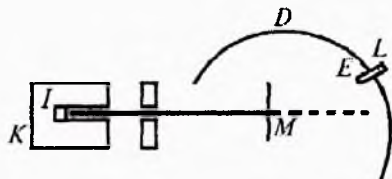
5- rasm. \alpha - zarrachalarning yupqa metallar pardadan o'tishi.
