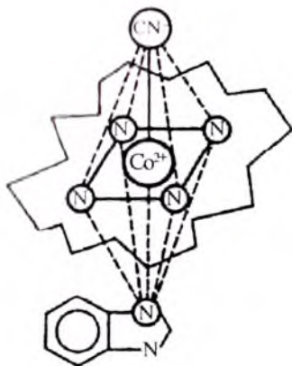
28-rasm. Vitamin B 12 yoki siankobalamin molekulasining tuzilishi.
