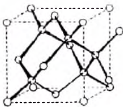
40-rasm. Olmos kristall panjarasining tuzilishi.
