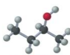
sec-butyl alcohol or s-butyl alcohol
