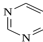
pirimidin
