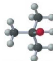
tert-butyl alcohol or t-butyl alcohol
