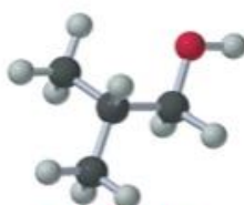
isobutyl alcohol
